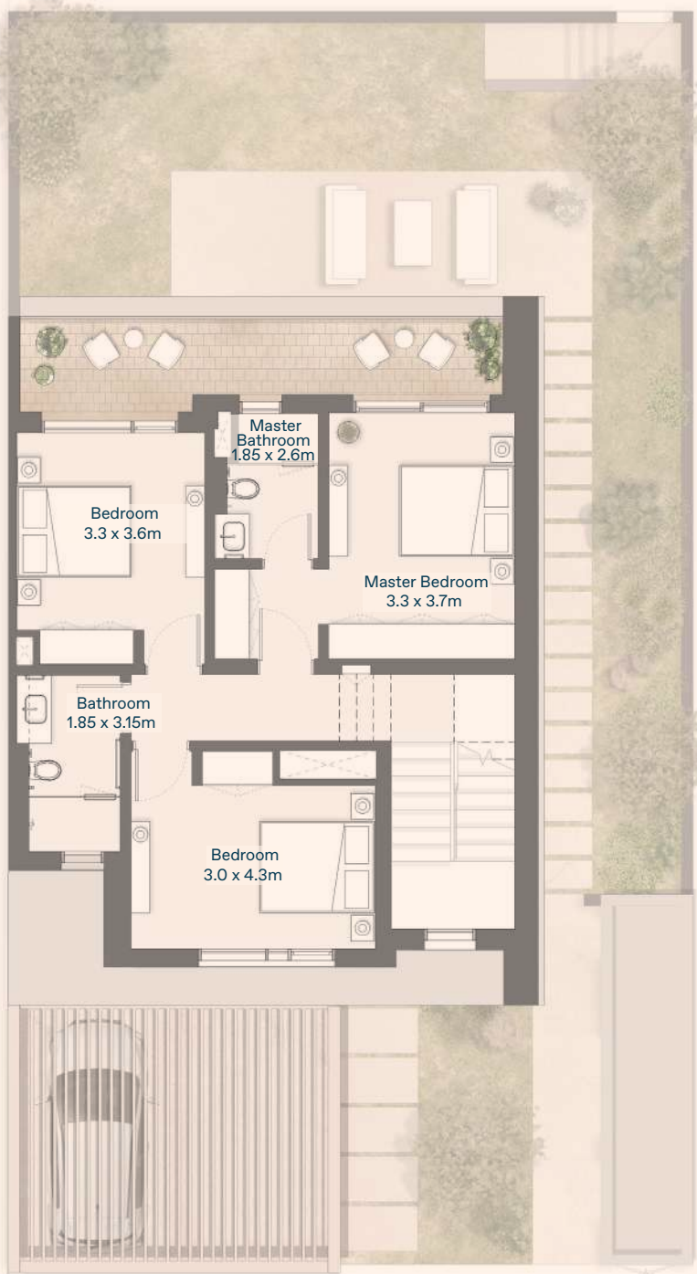
First Floor
